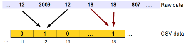
Figure 2: Example of formatting raw alert sequences into presence/absence data
