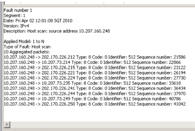
Figure 5: Traffic Aggregation Information Details Log
