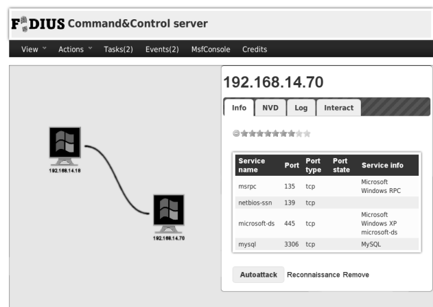
Figure 3: Screenshot of the FIDIUS Command&Control server
