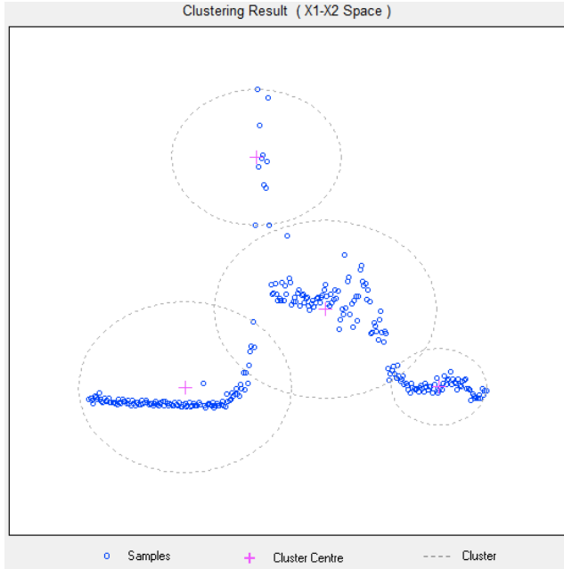
Figure 4: ECM Results Clustering ICMP Traffic
