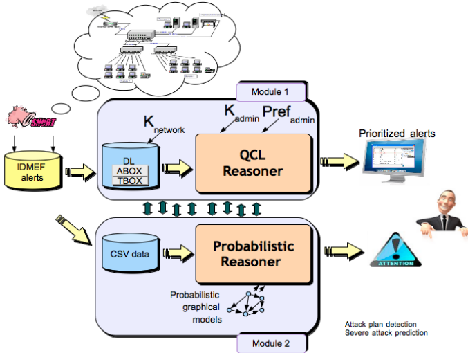
Figure 1: Building blocks of our alert correlation system
