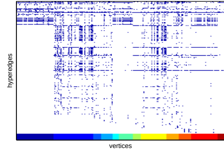
Figure 6: A spy plot of the hypergraph for user affiliation identification. Each vertex represents a user, and each hyperedge denotes a set evidence. There is a dot if the user is included in the set evidence. The vertices are sorted by labels and different colors on the bottom indicate the labels.
