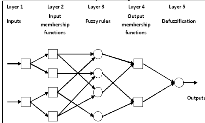
Fig 3: The structure of a neuro-fuzzy system
