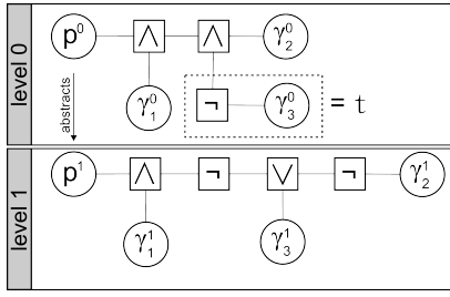
Figure 1: Example of a pattern with constraints and their abstractions.
