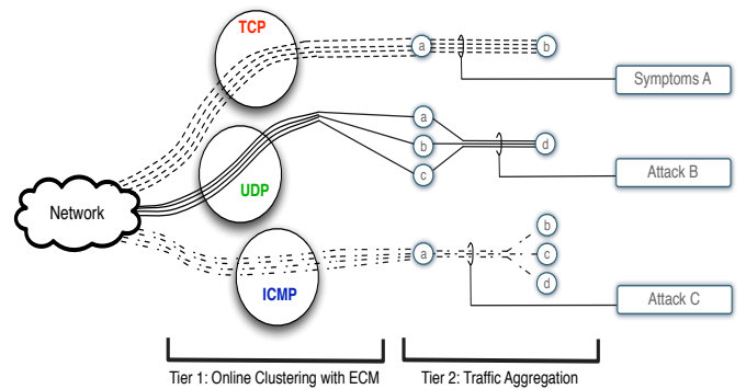
Figure 2: Online Two-tier Traffic Aggregation using ECM
