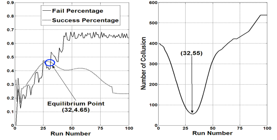
Figure 1: Pure Strategy Nash Characteristics.
