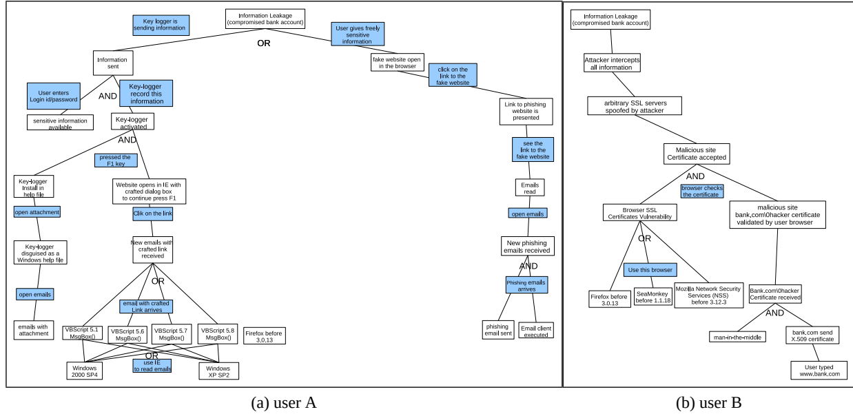
Figure 5: The resulting attack graphs for two hypothetical users after applying their profiles (see text for details).
