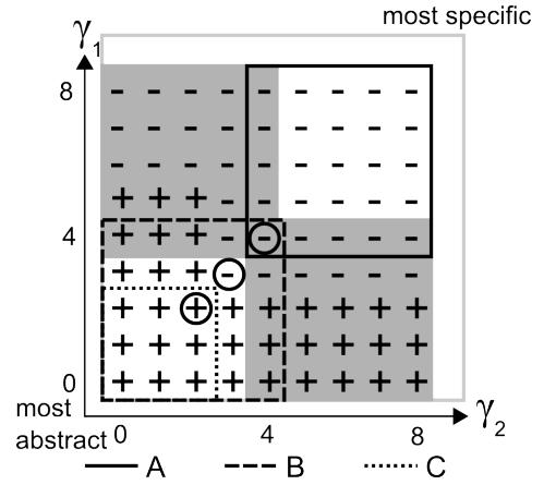
Figure 2: Example of the Pareto algorithm.
