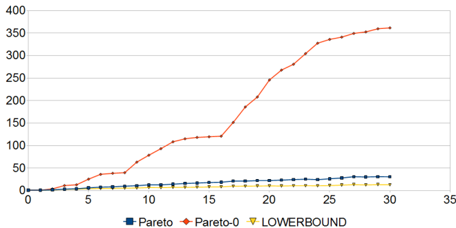
Figure 3: DL Reasoner calls in the two dimensional case. The x-axis represents the amount of possible abstractions and the y-axis the amount of reasoner calls.
