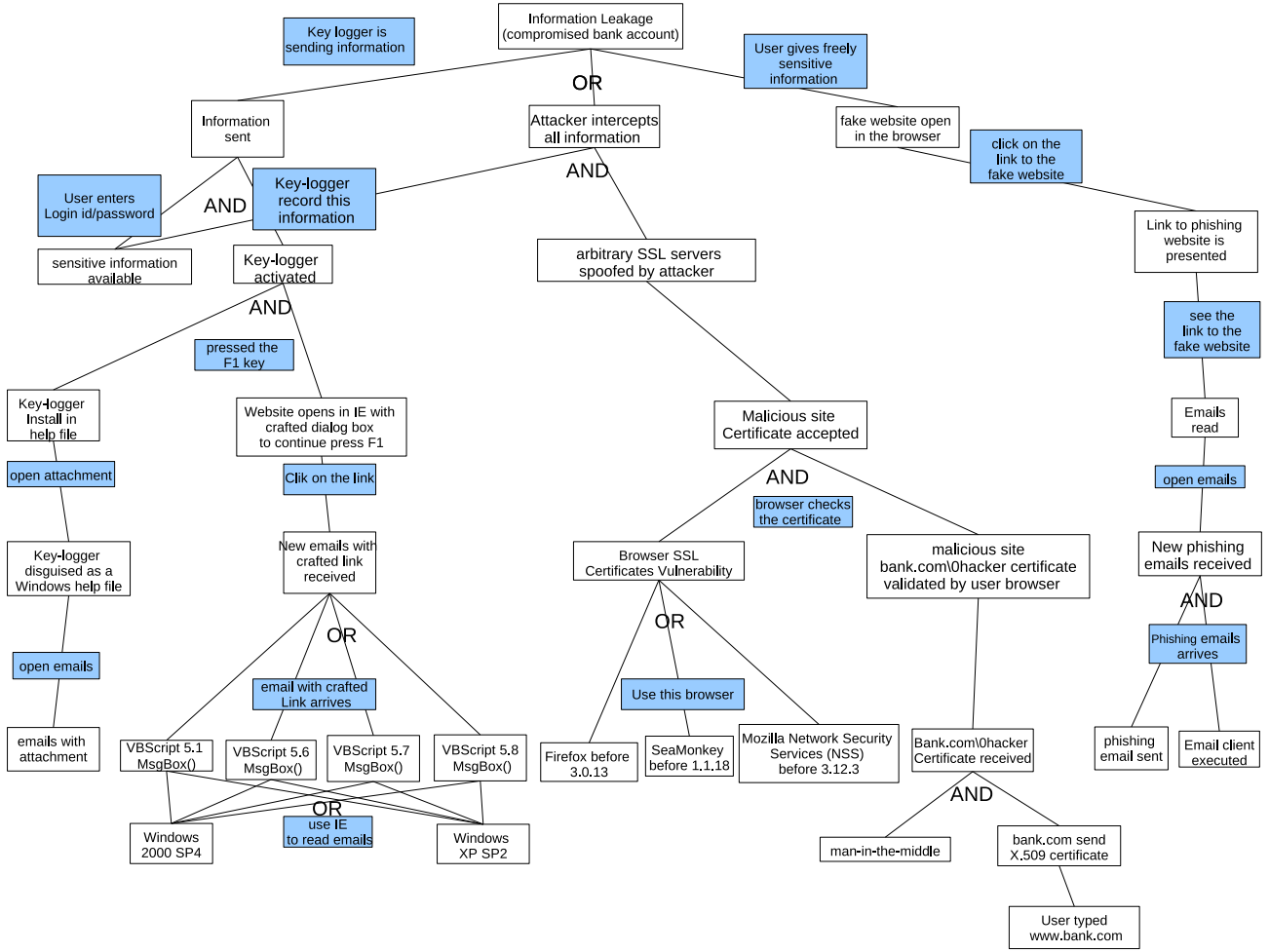
Figure 2: An instantiated attack graph augmented with user actions. This example graph shows three attack scenarios for how a user’s bank account credentials can become compromised. The leftmost subgraph is a keylogger attack, the middle subgraph is a SSL spoof attack, and the right subgraph is a phishing attack.
