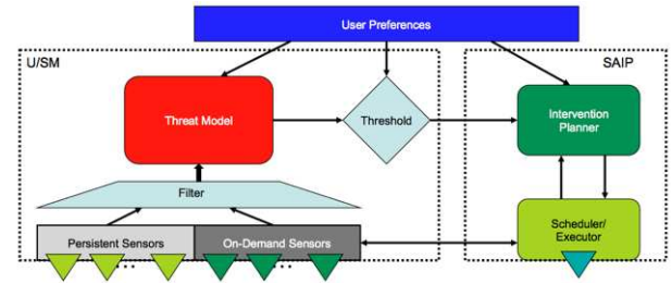
Figure 1: The proposed Mixed Initiative Planning and Scheduling Agent (MIPSA) Architecture.
