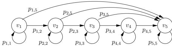
Figure 7: Markov Chain modeling an application’s updating process. Vertices are marked with version numbers, and edges with transition probabilities per time step.
