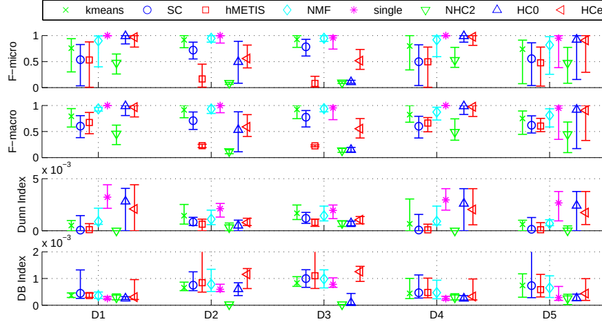
Figure 4: Performance of different algorithms on synthetic datasets. The parameters of the datasets are D1: \alpha = 2, \beta = 0 , D2: \alpha = 2, \beta = 0.05 , D3: \alpha = 2, \beta = 0.1 , D4: \alpha = 5, \beta = 0 , D5: \alpha = 10, \beta = 0 . For each dataset the performance is averaged on 50 trials. The maximal and minimal values are also shown in the figure.
