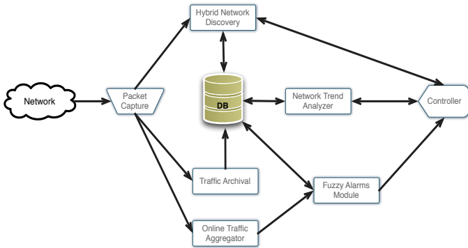
Figure 1: Combined Approach General Architecture
