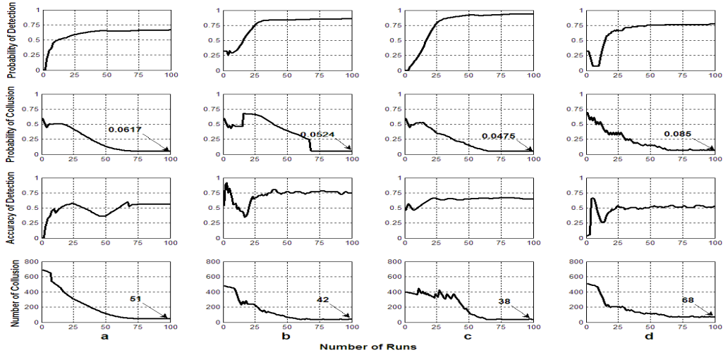
Figure 2: Mixed Strategy Nash Characteristics where in column (a) w_c = 20\% , in column (b) w_c = 40\% , in column (c) w_c = 60\% , and in column (d) w_c = 80\% .
