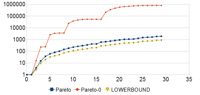
Figure 4: DL Reasoner calls in the four dimensional case with logarithmic scaling. The x-axis represents the amount of possible abstractions and the y-axis the amount of reasoner calls.
